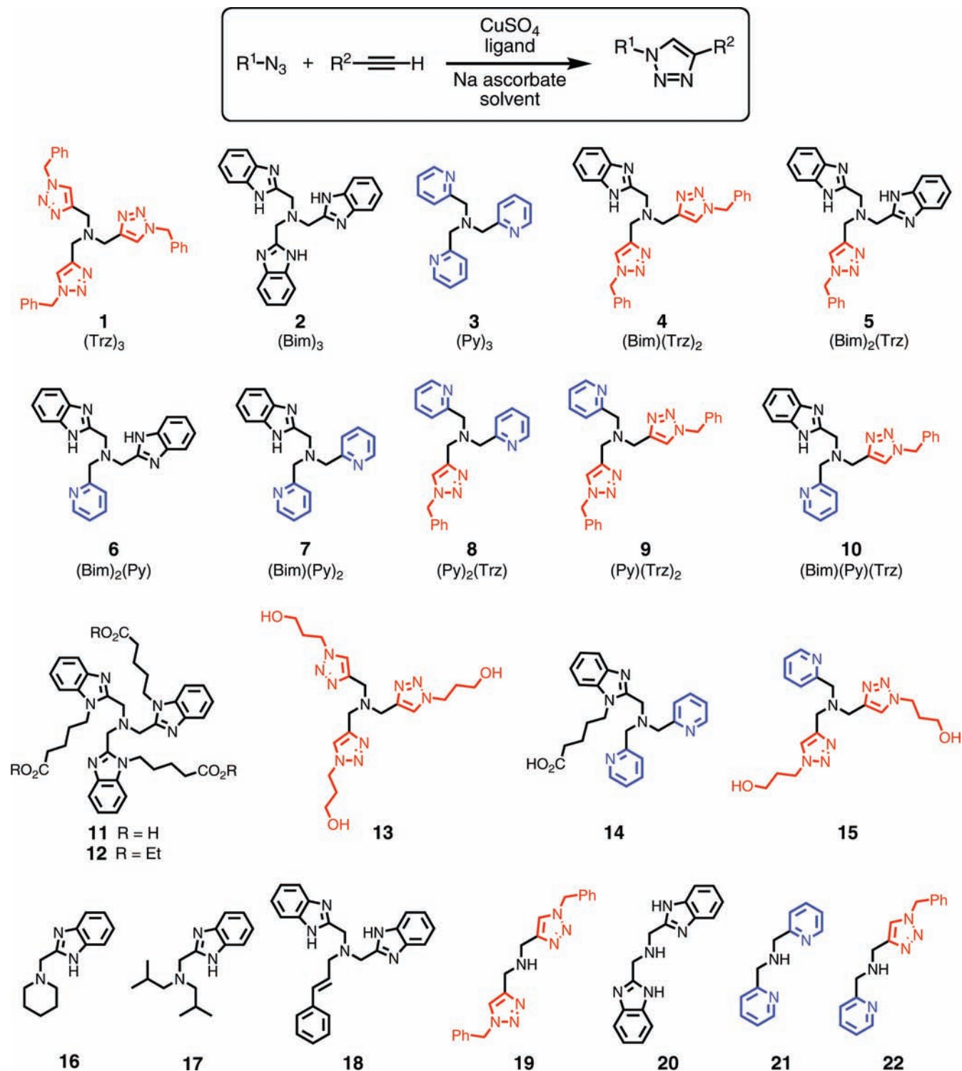
Figure 1. Ligand structures. (1–3) “Parent” ligands for CuAAC reactions. (4–10) “Hybrid” ligands based on 1,4-triazole (red), benzimidazole (black), and pyridine (blue) groups. (11–13) Ligands previously shown to be strongly accelerating. (14, 15) Modified hybrid ligands. (16–22) Truncated ligands containing fewer than three heterocyclic arms. Abbreviations below the compound numbers refer to the nature of the heterocyclic arms: Trz = triazole, Bim = benzimidazole, Py = pyridine.
