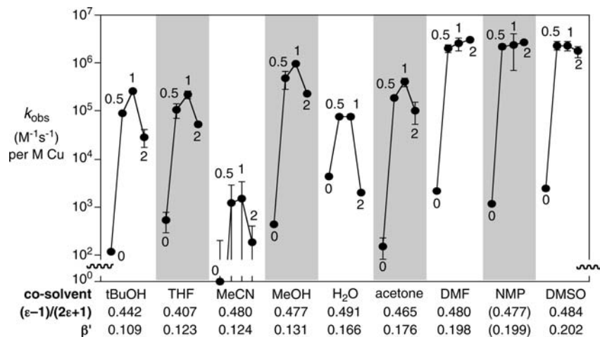
Figure 5. CuAAC rates with variations in solvent and ligand:metal ratio. Observed second-order specific activities for reactions accelerated by Cu•7 in 20% H 2 O, 10% DMSO, and 70% polar organic cosolvent. [CuSO 4 ] = 50 \mu M, [7] = variable, [BnN 3 ] = 100 \mu M, [PhCCH] = 200 \mu M. The ligand:Cu ratio in each solvent was varied from 0 to 2, as indicated. The donor abilities of the polar organic cosolvent are given by the basicity parameter \beta' (representing the free energy of potassium ion transport corrected for solvent polarity). 12b Values for NMP were estimated from data reported in ref 12a.
