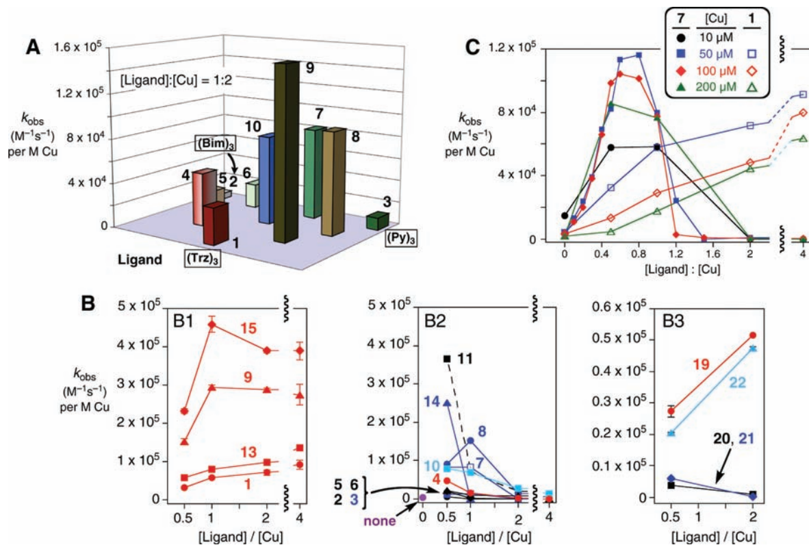
Figure 3. Reactions in 9:1 H 2 O:DMSO. (A) Observed second-order specific activities: [BnN 3 ] = 100 μM, [PhCCH] = 200 μM, [CuSO 4 ] = 50 μM, [Ligand] = 25 μM. (B) Comparison of hybrid ligands at different ligand:copper ratios under the same conditions. The ligands are grouped by class and color coded according to their heterocyclic content: black = two or three benzimidazoles in the structure; dark blue = two or three pyridines; red = two or three triazoles; light blue = one of each heterocycle. (C) Comparison of ligands 7 and 1 under bioconjugation conditions.
