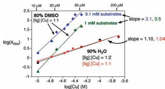
Figure 6. Determination of rate order in [Cu•7] in 4:1 and 1:9 mixtures of DMSO:H 2 O. [Cu] was varied from 10 to 200 \mu M, [7] was varied according to the given ratio, [BnN 3 ] = 100 \mu M or 1 mM in 80% DMSO and 100 \mu M in 90% H 2 O, [PhCCH] = 2[BnN 3 ]. In 80% DMSO, the reactions containing <20 \mu M Cu stopped before completing many turnovers, so initial rates are reported for these experiments. The correlations for reactions in 80% DMSO should therefore be regarded as approximate determinations of catalytic rate order.
