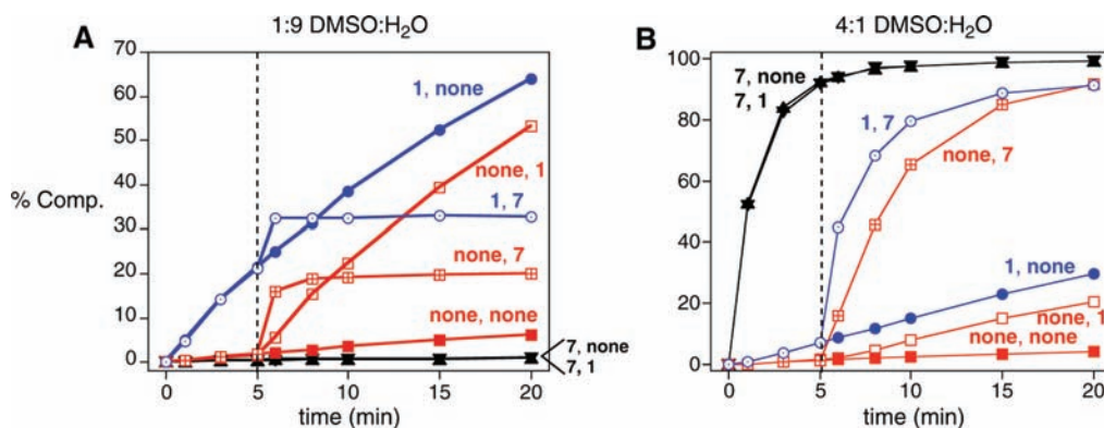
Figure 4. Sequential ligand addition experiments. (A) CuAAC reactions in 10% aqueous DMSO were initiated with 50 μM CuSO 4 and 100 μM of the first indicated ligand. At 5 min, a concentrated solution of the second ligand was added to a final concentration of 100 μM (vertical dotted line). (B) As in part A with reactions performed in 80% DMSO. For both sets of experiments, [BnN 3 ] = 100 μM, [PhCCH] = 200 μM.
