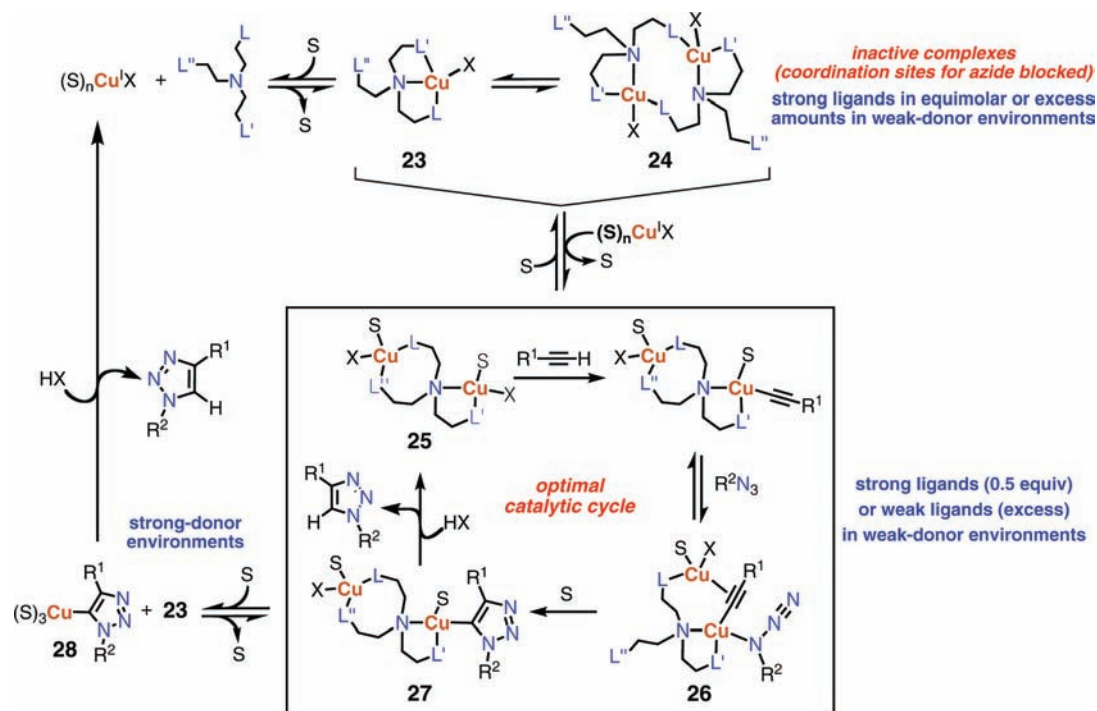
Figure 7. Proposed mono- and binuclear speciation in the CuAAC process. X = anionic donor such as \sigma -acetylide, halide, hydroxide, or triazolide; S = neutral intermolecular donor such as DMSO, other solvent, \pi -alkyne, or organic azide. Productive complexes are not formed when only one heterocyclic donor arm (L) exists.
